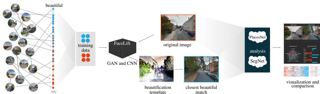
Figure 1. An illustration of the FaceLift framework. The training data of urban scenes with beautiful and ugly labels is fed into the FaceLift algorithms (the generative adversarial network and convolutional neural network models). These transform the original image into its beautified version. The two images—original and beautified—are compared in terms of urban elements that have been added or removed.
