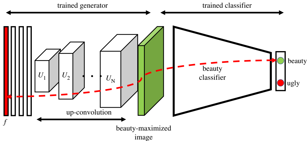
Figure 5. Architecture of the synthetic beauty generator. This consists of a generator of synthetic scenes concatenated with a beauty classifier. The green block is the beauty-maximized template \hat{I}_j , which is subject to forward and backward passes (red arrow) when optimizing for beauty.
